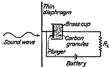
Circuit illustrating the action of a single-button carbon-granule transmitter as used in a telephone handset or a carbon microphone.
